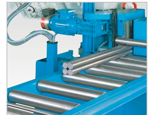
A bundle vise is provided for cutting entire material packs to length
